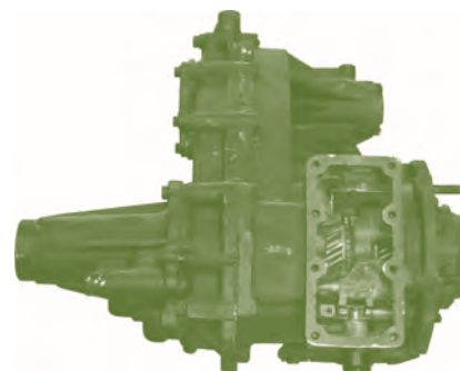
Caja transfer Suzuki Grand Vitara
